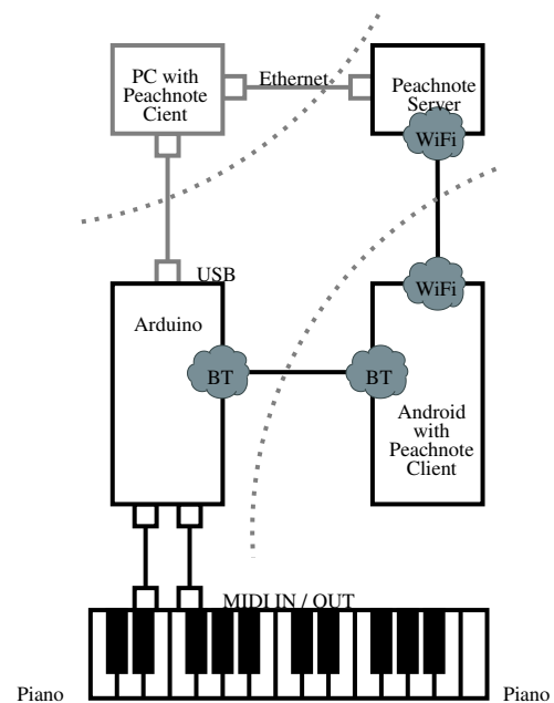
Figure 1. The Peachnote Piano components: a MIDI keyboard (below), a custom built MIDI to Bluetooth (BT) bridge (center left), a smartphone with a Peachnote Piano client (center right) and the Peachnote Piano server (top right). The greyed out part is a PC with a Peachnote Piano client.
